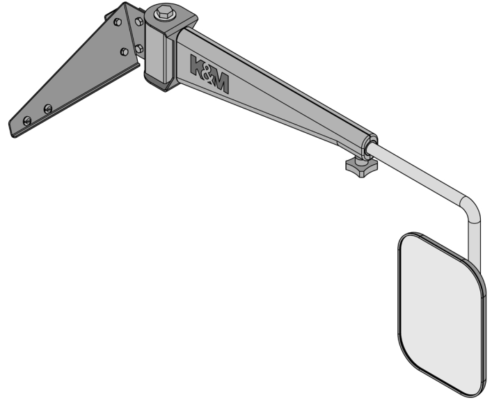
PN: 3134 VIEW WITH BRACKET
