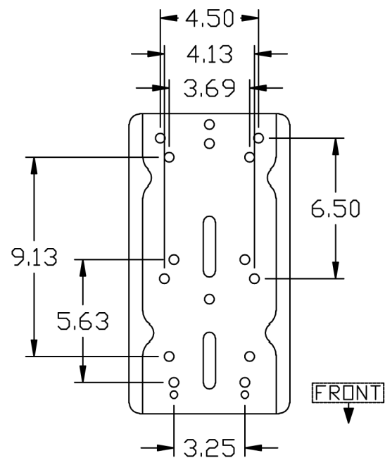
BOLT PATTERN
