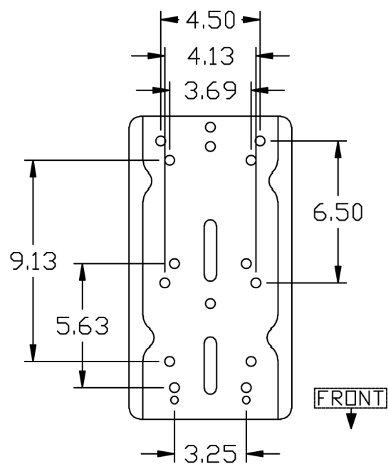
BOLT PATTERN
