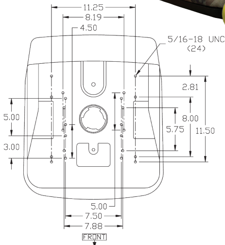
Drawing shows the mounting patterns for PN 7927, 7937 and 8135.
