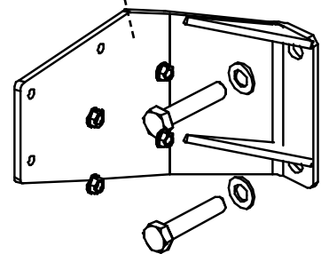
Part 1 of 2 New Holland BOA 28" LH Bracket
