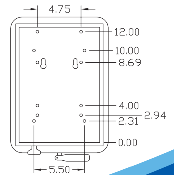
MSG83 BOTTOM VIEW
