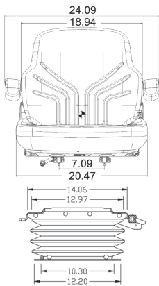
FRONT VIEW PN: 6977
