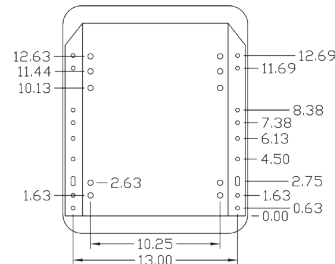
TOP VIEW PNs: 6551 & 6553
