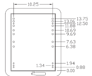
BOTTOM VIEW PNs: 6551 & 6553
