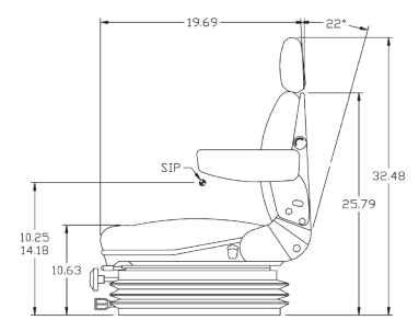
SIDE VIEW PN: 6545
