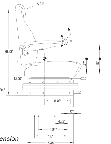
SIDE VIEW PNs: 6423 & 6424
