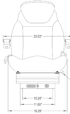
FRONT VIEW PNs: 6423 & 6424
