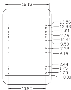
BOTTOM VIEW PNs: 6550 & 6552
