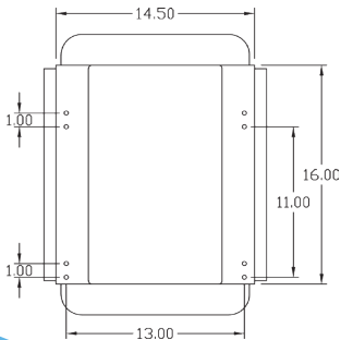
TOP VIEW PNs: 6550 & 6552
