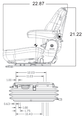
SIDE VIEW PN: 6977
