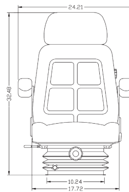
FRONT VIEW PN: 6545
