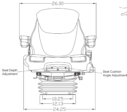
FRONT VIEW PNs: 6906 & 6907
