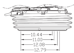
SIDE VIEW PNs: 6906 & 6907
