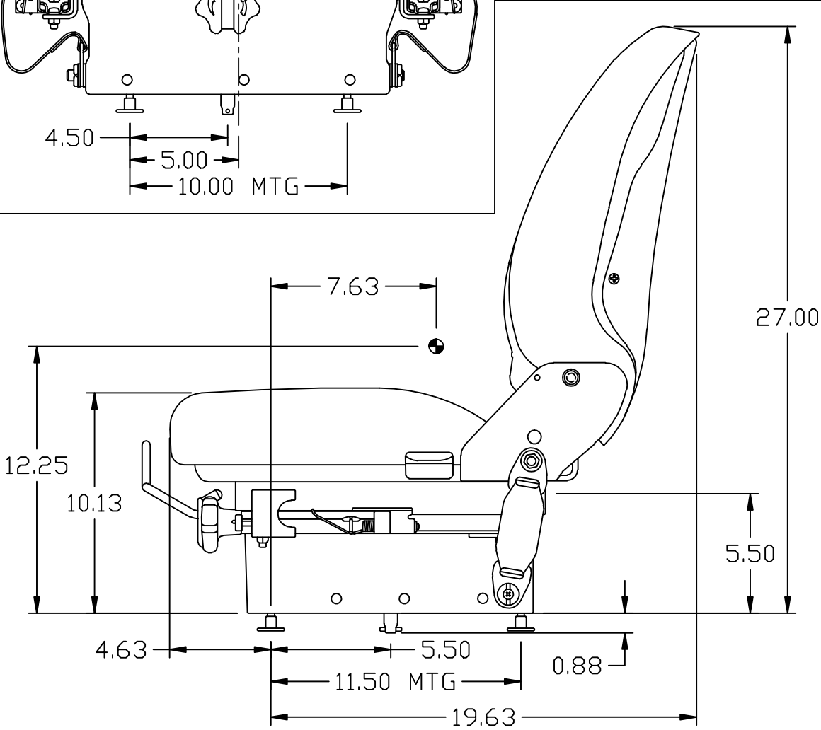
Side View
